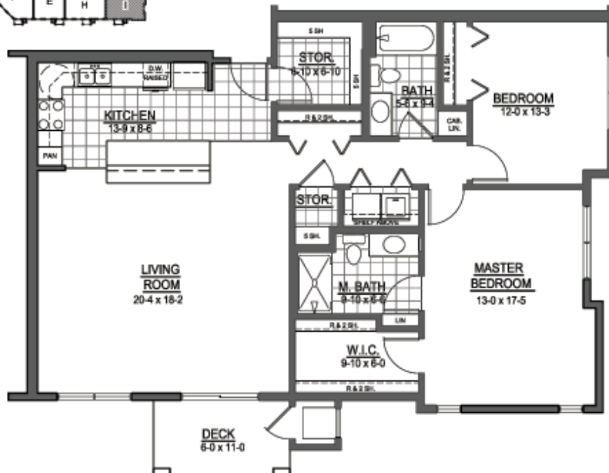
Unit I 2 Bedroom, 2 Bath - 1397 Sq. Ft. SCALE 1/8"=1'-0"
